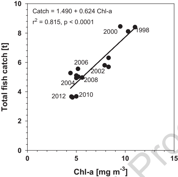
Fig. 20.7 Dependence of total fish catch (tons) on phytoplankton chlorophyll-a (mg m -3 ) for the post-restoration years (1998ff.). Chl-a data from DWS-Hydro-Ecology, total fish catch data from Austrian Fishery Association
